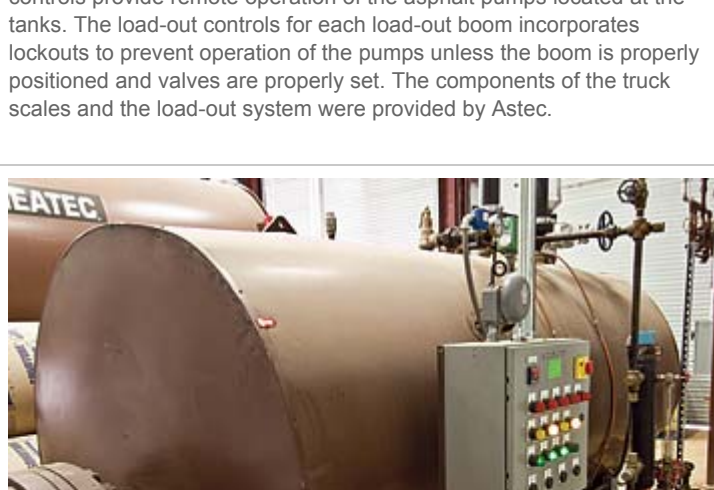
Steam Generator A steam generator turns water into steam—and that steam is used to heat tank cars. The generator is located in the enclosed building alongside the hot-oil heaters. Its source of heat is the thermal fluid that is heated by the hot-oil heaters.
