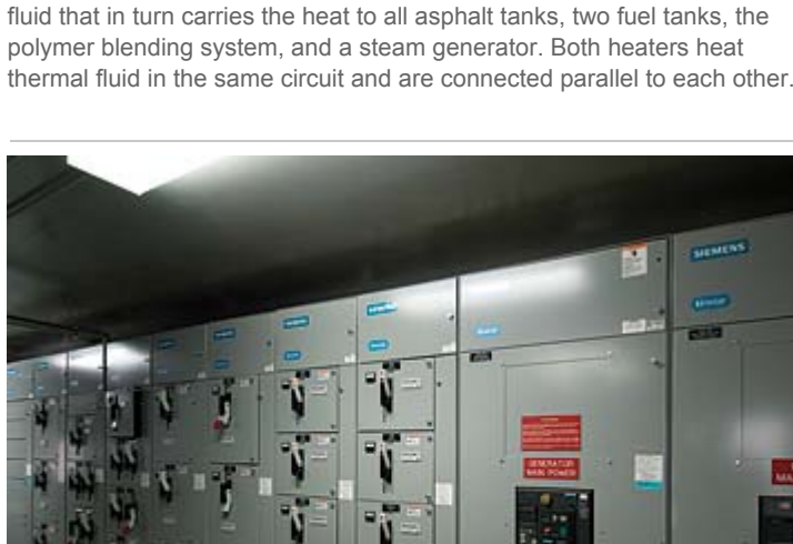
Motor Control Center The control center centralizes all electrical power for the terminal and for the motor controls. The controls are housed in a series of electrical racks and panels. Electrical power is sub-divided into two independent control systems, one for the polymer blending system and another for all other electrical power. A computer is also located in the motor control center. It controls the asphalt pumps used to transfer asphalt from one tank to another. Positions of the three valves on the outlet side of each asphalt pump can be verified on the computer screen before the pump is operated.
