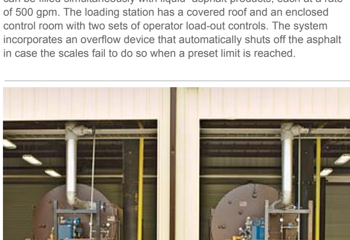
Hot-Oil Heaters Two hot-oil heaters are located in an enclosed building. Each heater has an output of 8 million Btu/hour. The building has space for a third heater if needed for future expansion. The heaters have refractory lining that enables them to burn a variety of heavy fuels or waste oils, in addition to No. 2 diesel fuel. They have combination burners that also enable them to burn natural gas as an alternative fuel. The two heaters heat thermal fluid that in turn carries the heat to all asphalt tanks, two fuel tanks, the polymer blending system, and a steam generator. Both heaters heat thermal fluid in the same circuit and are connected parallel to each other.
